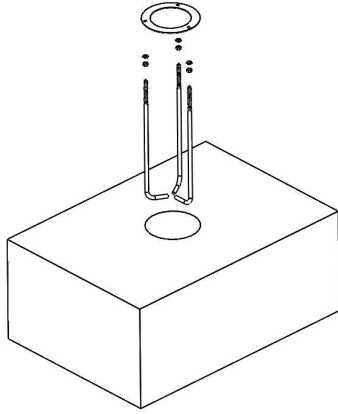
1.1 Ankaraj, zemine beton dökülerek sabitlenir. 1.1 The anchorage is fixed by pouring concrete into the ground.
