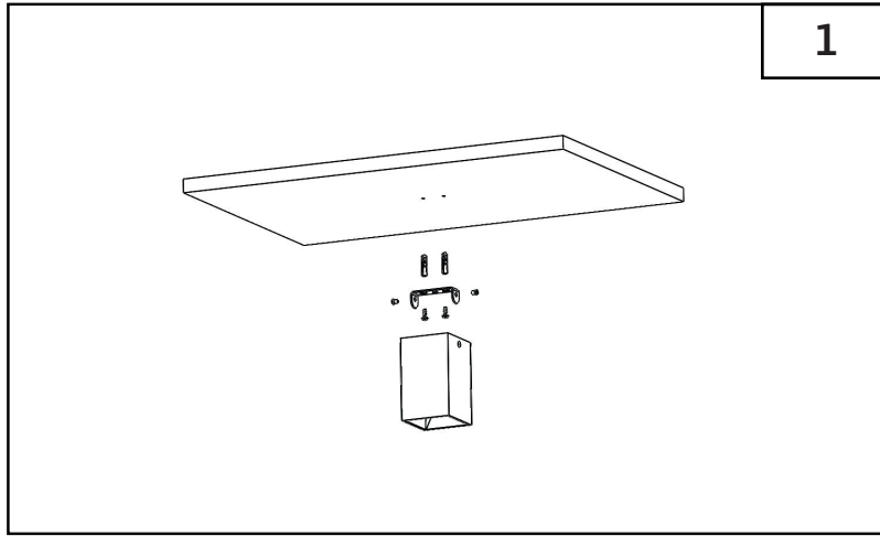
1.1 Ölçülere uygun bağlantı delikleri delinir.Ürün kasası civatarla tavana monte edilir. 1.1 Connection holes are drilled in accordance with the dimensions. The product casing is mounted to the ceiling with bolts.
