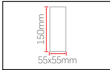
1.1 Ölçülere uygun bağlantı delikleri delinir.Ürün kasası civatarla tavana monte edilir. 1.1 Connection holes are drilled in accordance with the dimensions. The product casing is mounted to the ceiling with bolts.
